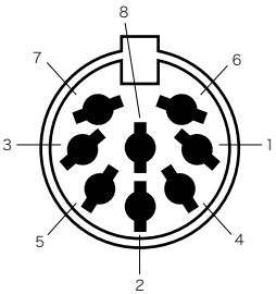
Figure seen from the cable side (TC-1/TC-5)
