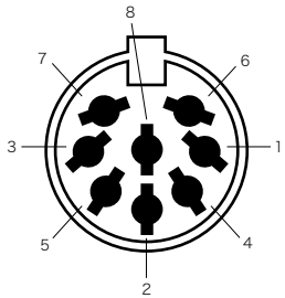
Figure seen from the cable side (TC-1/TC-5)
