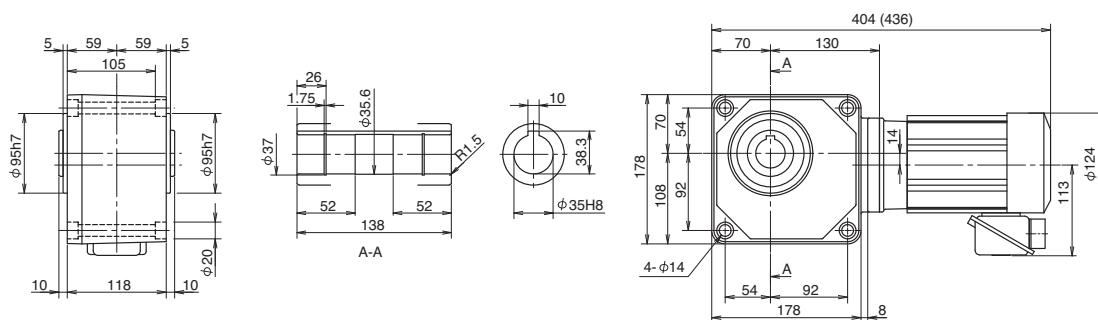
Fig. 4 Designate model and voltage and frequency when ordering. Brackets contain dimension, model, or mass of type with brakes. RNYM05-1430-80~240 Mass 16kg (RNYM05-1430-B-80~240) (Mass 17kg)
