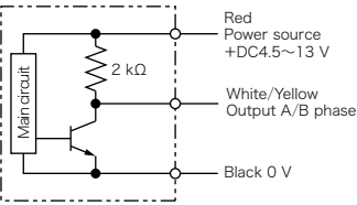
Voltage output type S, C, O
