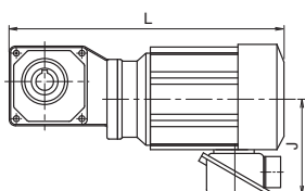
Fig. 1 0.1~0.2kW Without brake
