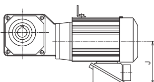
Fig. 3 0.4~1.5kW Without brake
